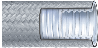
Convoluted Low Profile PTFE Lined Hose with Braided Stainless Steel Cover
